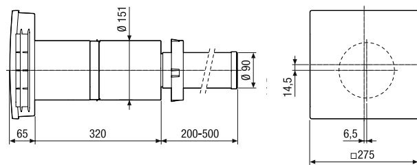
PPB 30 Endmontage-Set
